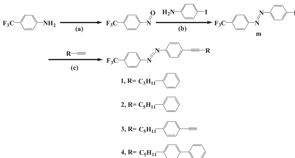
Scheme 1. Reagents and conditions: (a) Oxone, \text{CH}_2\text{Cl}_2 , \text{H}_2\text{O} , r. t., 15 h; (b) \text{AcOH} , r. t., 15 h; (c) TAE, THF, \text{PdCl}_2(\text{PPh}_3)_2 , \text{CuI} , \text{PPh}_3 , 30^\circ\text{C} , 10 h.
