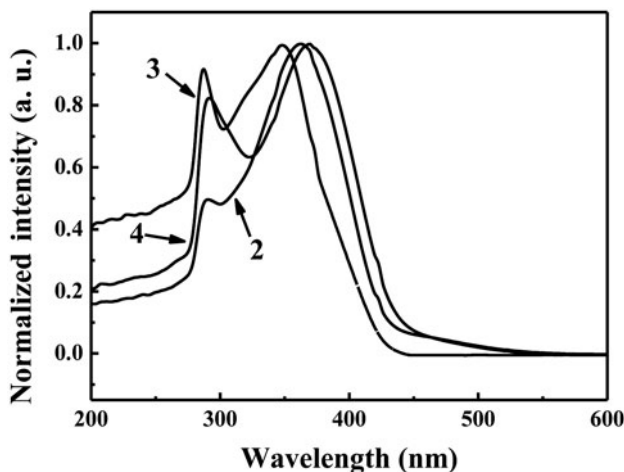
Figure 1. UV-Vis absorption spectra of 2–4 in \text{CH}_2\text{Cl}_2 under room temperature.
