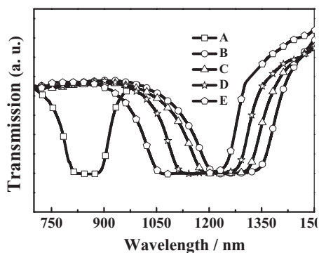
Figure 3. Dependence of the reflection band on the series compounds.
